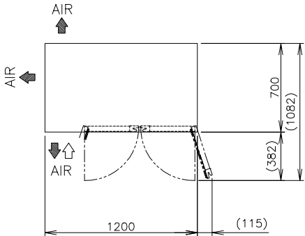
VIEW A(1/10)
