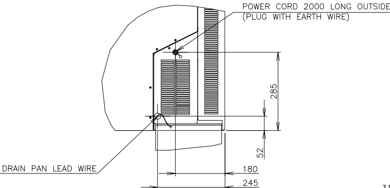
VIEW A(1/10)
